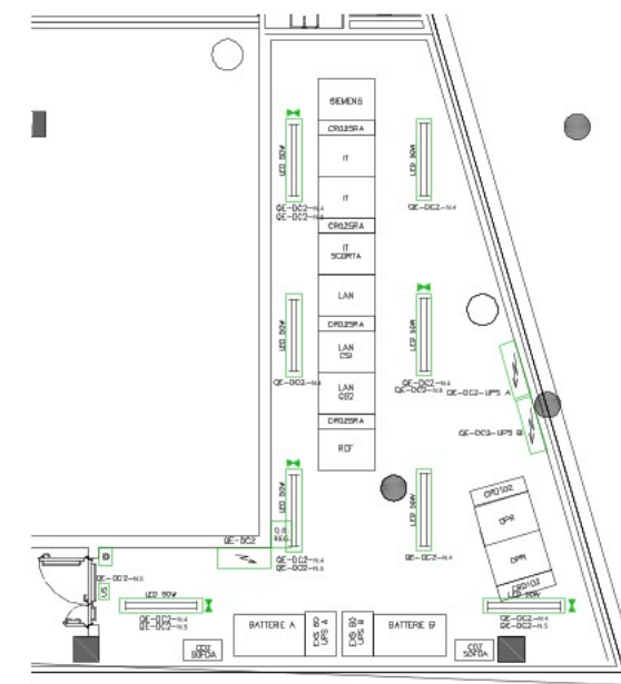
DATA ROOM - ILLUMINATION
