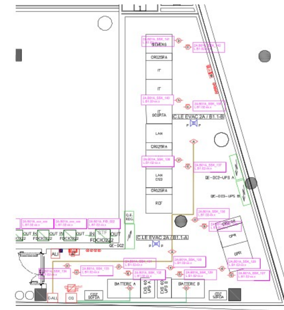
DATA ROOM - SAFETY DEVICES
