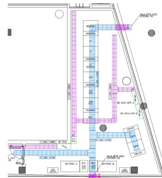
DATA ROOM - OVERHEAD DISTRIBUTION
