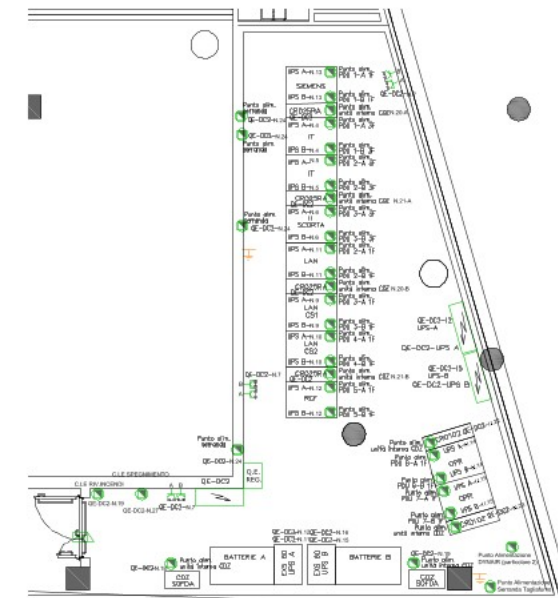
DATA ROOM - POWER SUPPLY
