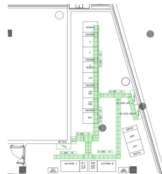
DATA ROOM - UNDERFLOOR DISTRIBUTION
